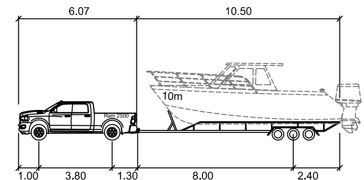
TYPICAL CAR/TRAILER UNIT
