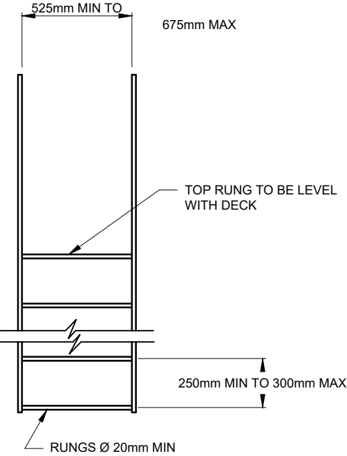
LADDER DETAIL
