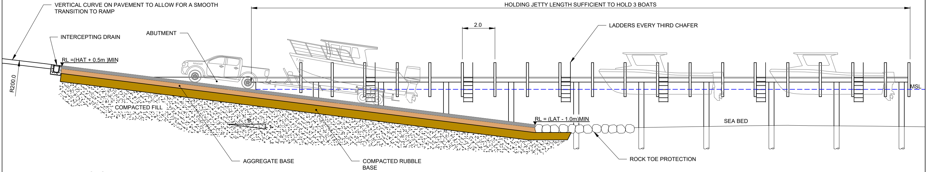
TYPICAL LONGITUDINAL RAMP SECTION
