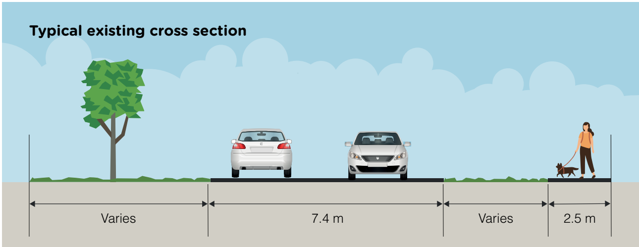
Safe active street cross section
