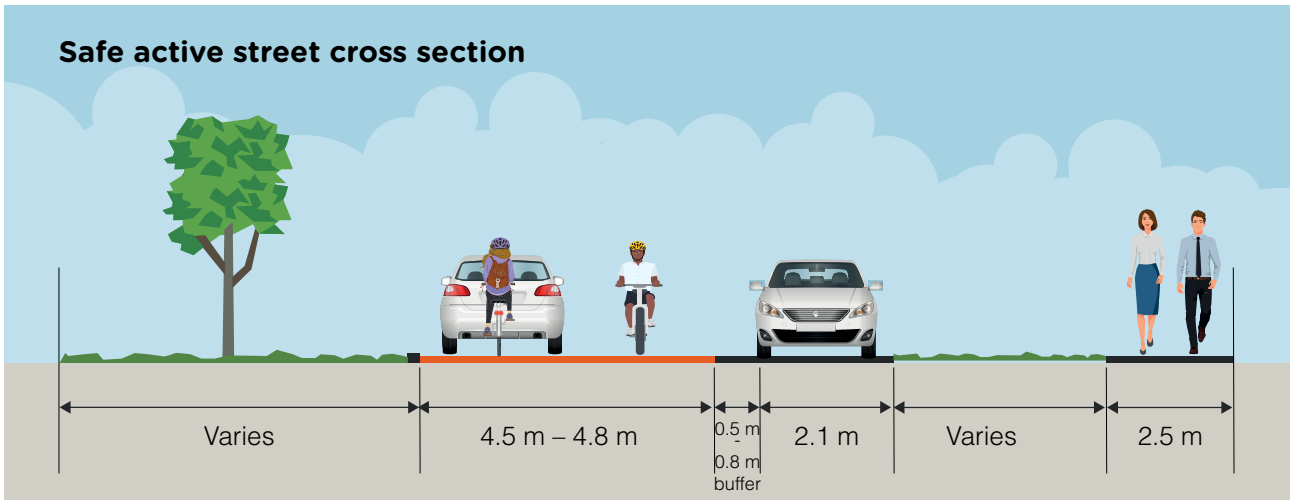
Safe active street cross section at slow points
