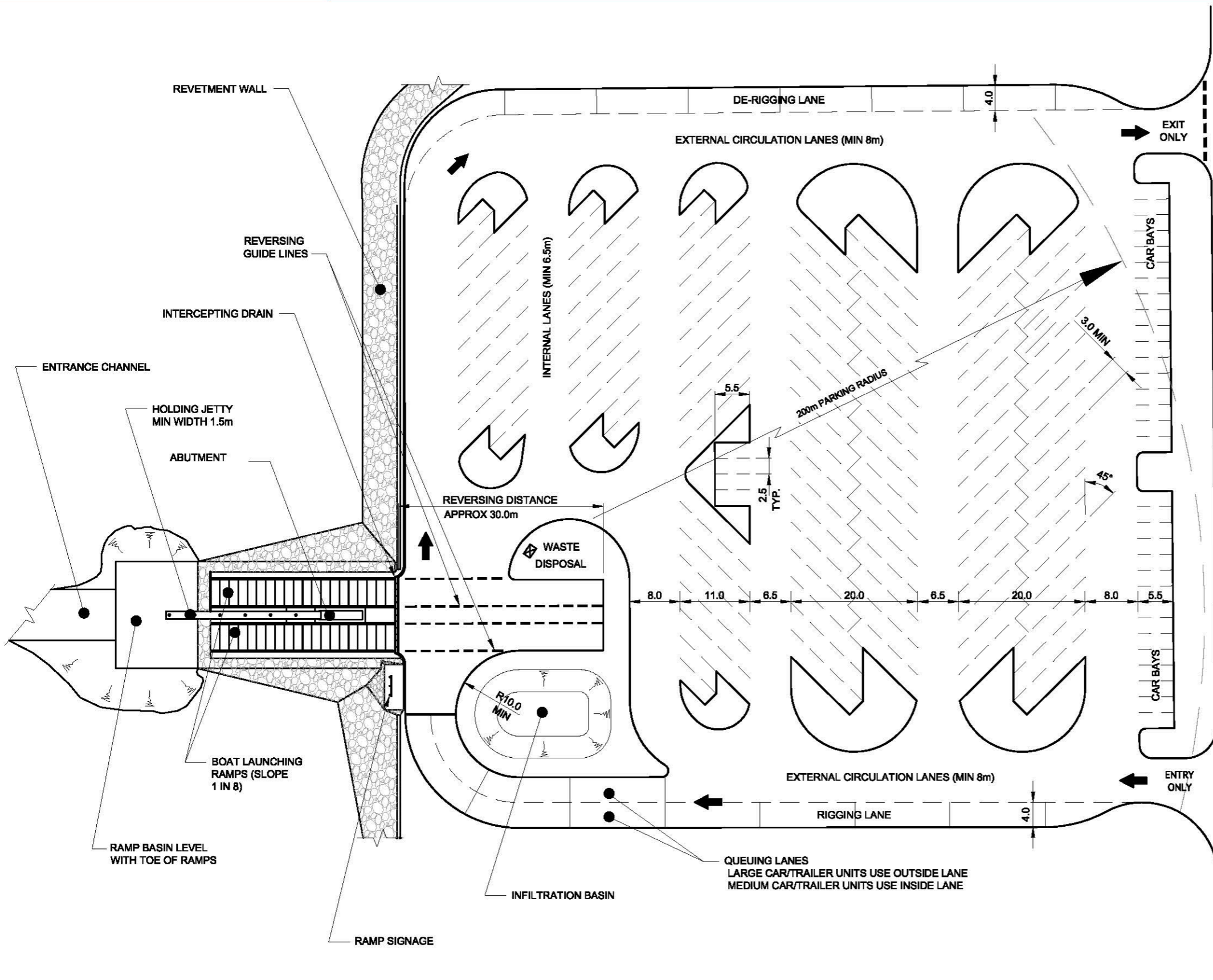
BOAT LAUNCHING FACILITY TYPICAL LAYOUT
