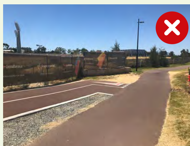
Figure 4.4 Examples of poor path intersection connections with no corner splays and sharp turn.
