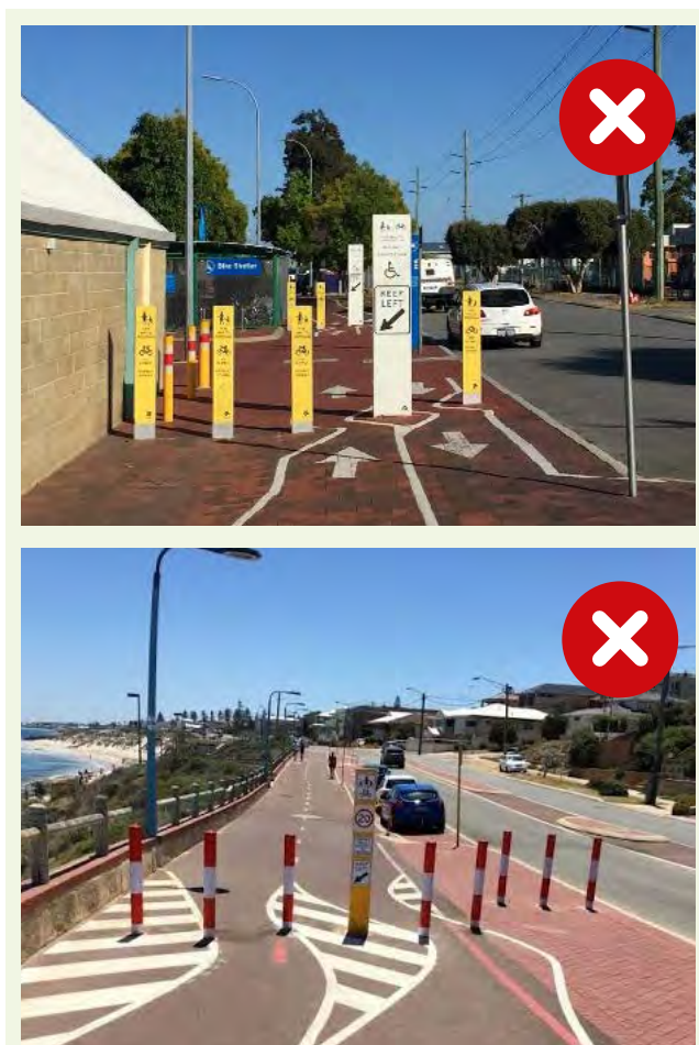
Figure 10.13 The use of bollards is not supported as a conflict management treatment on shared paths.
