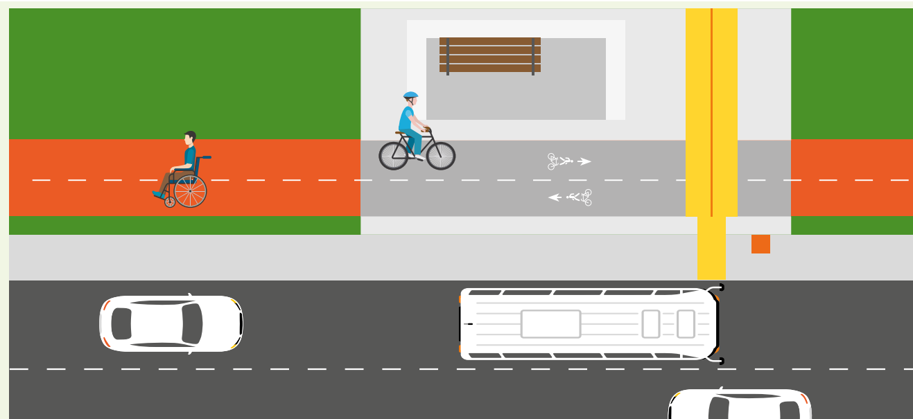
Figure 10.2 Shared path in front of bus shelter – acceptable in situations where both boarding/alighting and path volumes are low (or where no other option is available).
