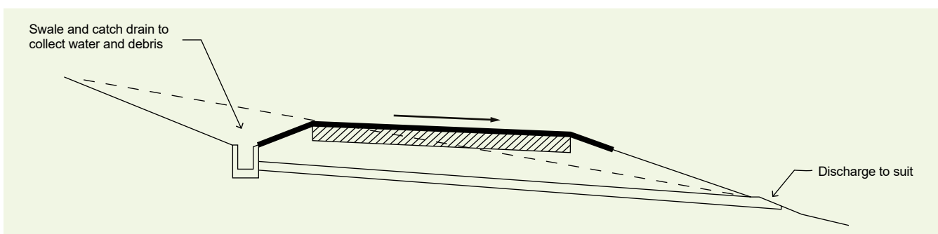
Figure 6.2 Drainage and crossfall requirements for path where existing terrain exceeds path crossfall – preferred (image courtesy of Austroads Guide to Road Design: Part 6A (Figure 5.14)).
