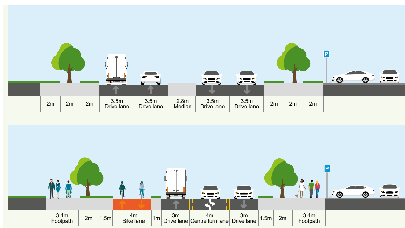
Figure 2.1 'Road diet' principles can be used to re-allocate road space to cycling infrastructure.
