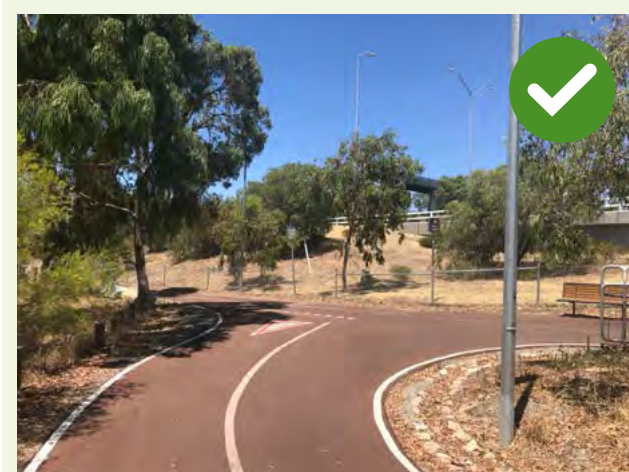
Figure 4.3 Examples of good path intersection connection with corner splays and turn radius.
