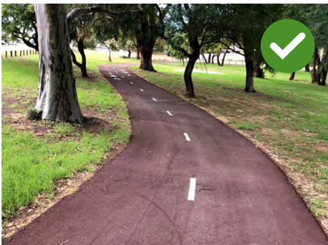
Figure 3.12 Example of clear sightlines across the inside of horizontal curves.
