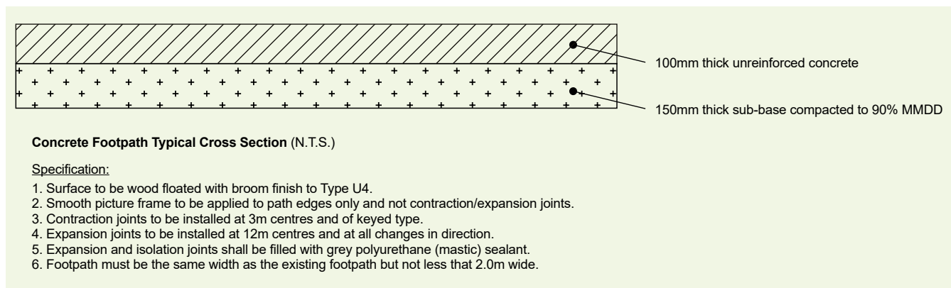
Figure 5.4 Typical pavement cross-section for concrete paths.
