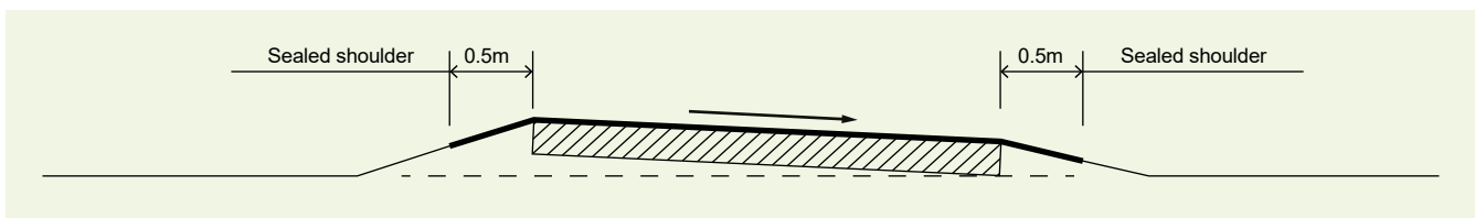
Figure 6.1 Drainage and crossfall requirements for elevated path in flat terrain (image courtesy of Austroads Guide to Road Design: Part 6A (Figure 5.14)).
