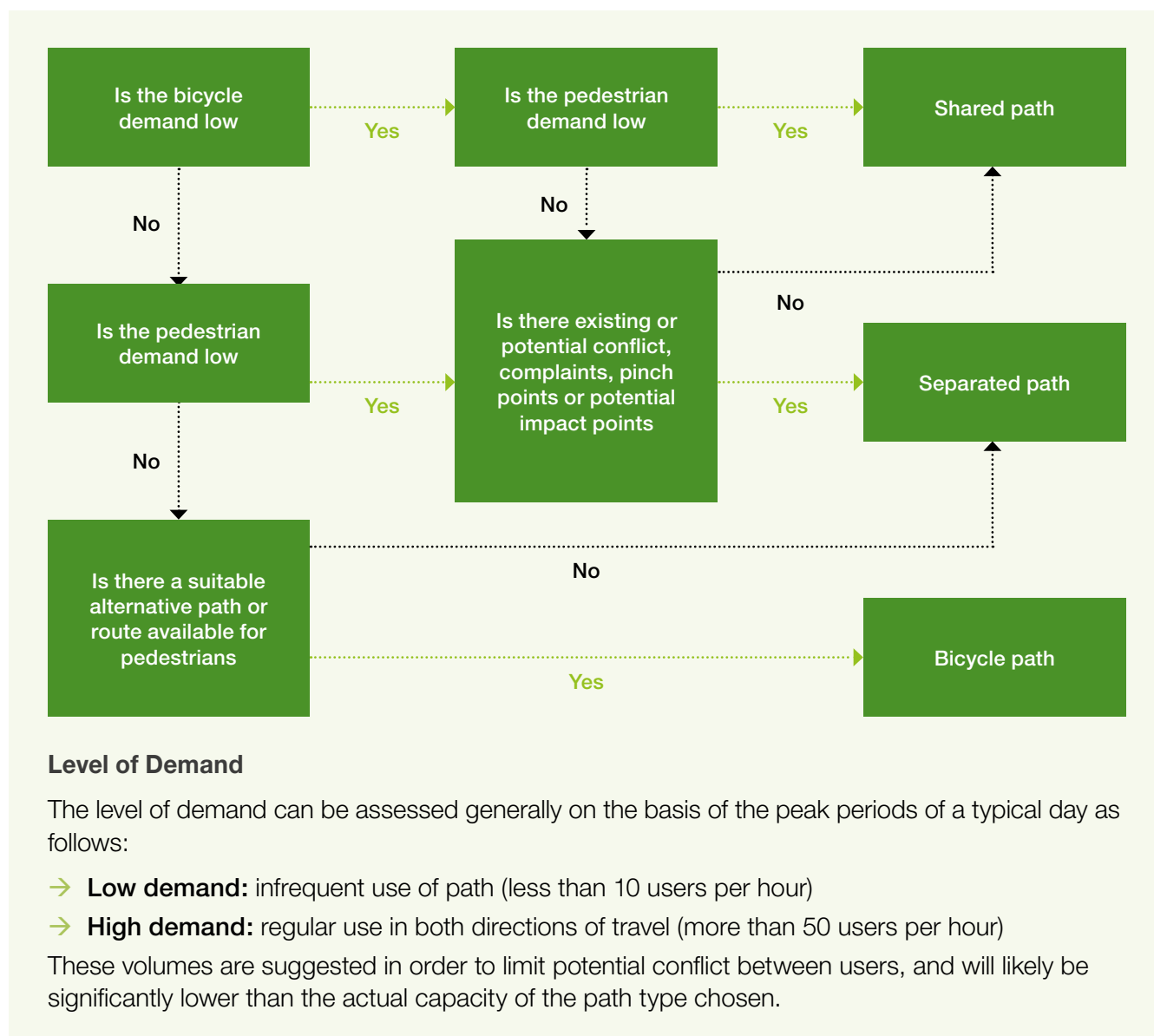
Figure 2.2 Path type decision making framework (image adapted from Austroads Guide to Road Design Part 6A ).
