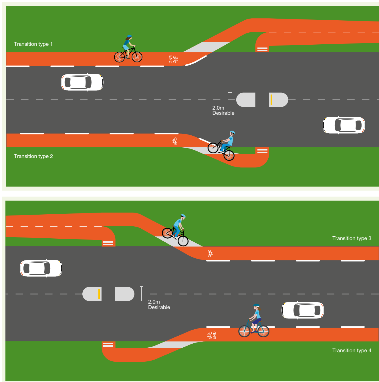
Figure 10.5 Transitions between on-road and off-road cycling infrastructure (indicative only).
