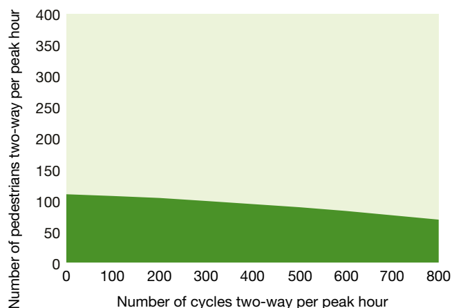
Figure 2.4 Separation criteria for path with 75:25 directional split – typical of paths which are popular with commuters (image adapted from Queensland Department of Transport and Main Roads 2015).
