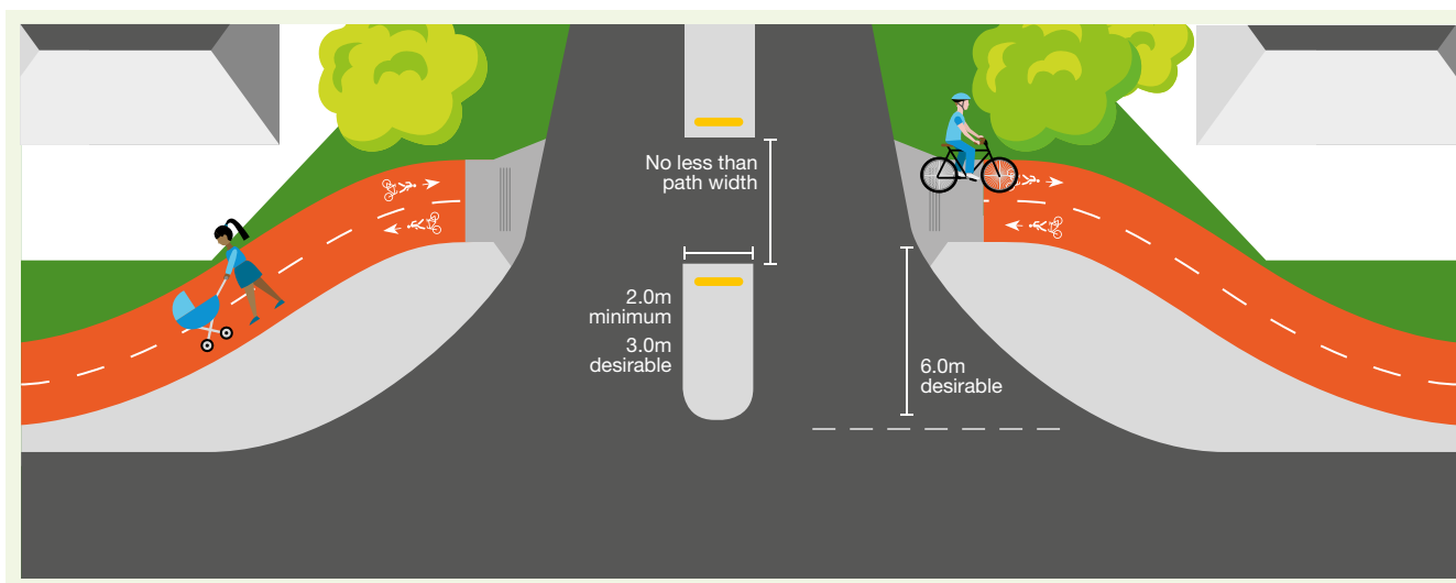
Figure 4.11 Preferred cut-through geometry.
