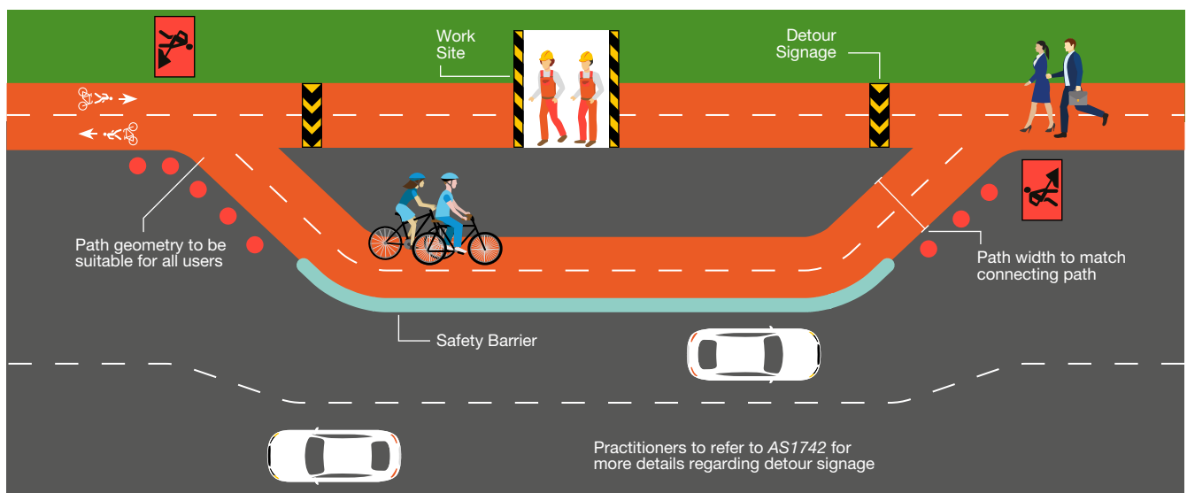
Figure 11.14 Example of a TMP used for a shared path diversion (image courtesy of Austroads Guide to Road Design: Part 6A).
