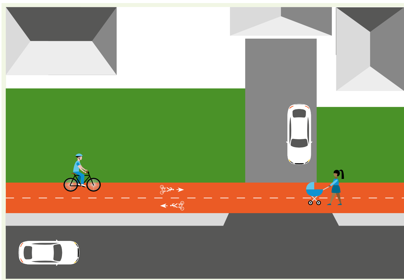
Figure 4.5 Intersection type 1 (non-indented, priority) – suitable only for driveways.
