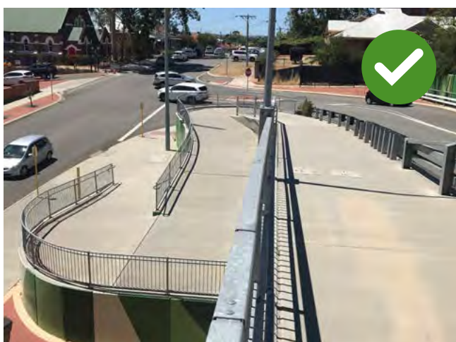
Figure 3.9 Example of the preferred curvilinear switchback.
