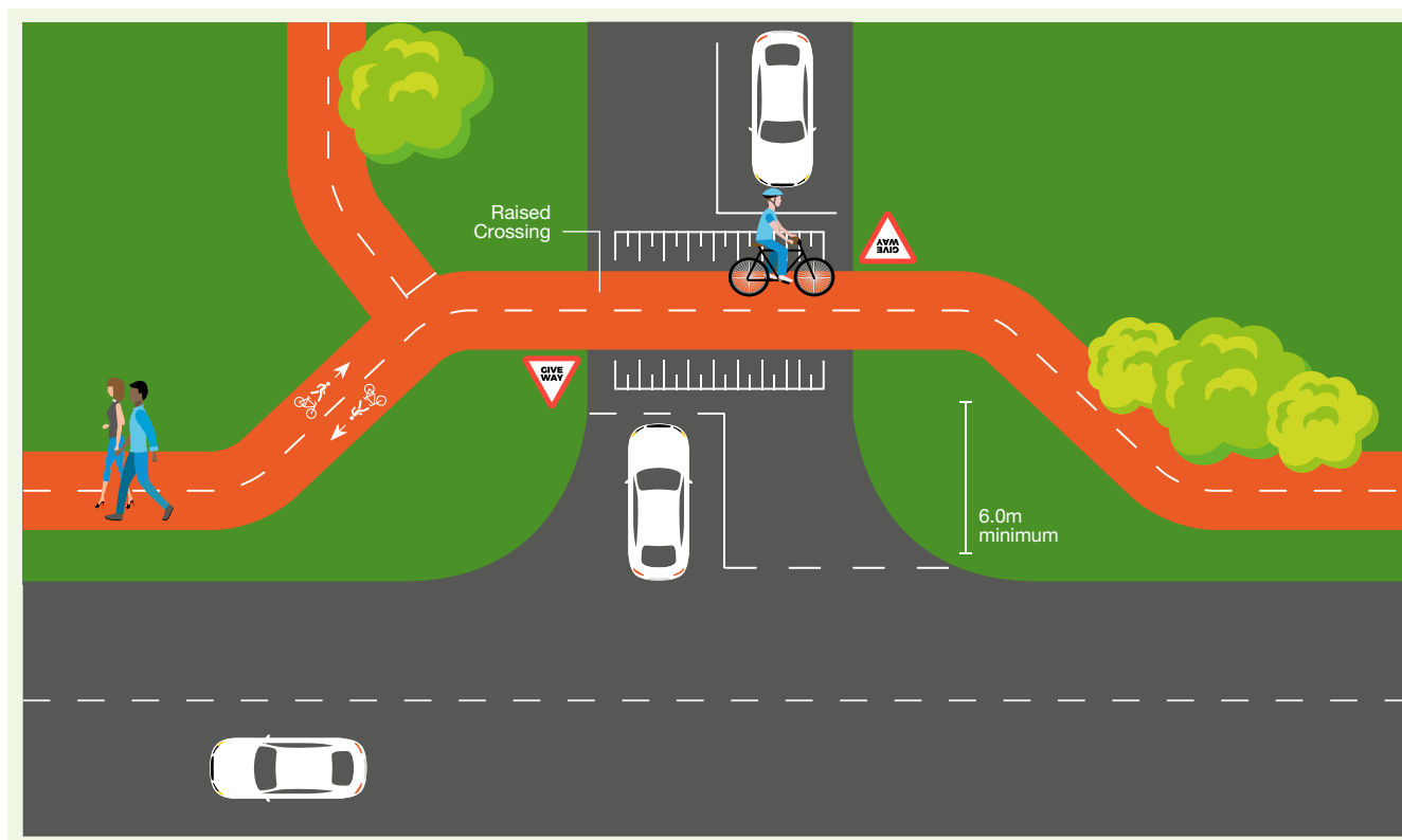
Figure 4.6 Intersection type 2 (indented, priority) – only for minor roads where sufficient sightlines and storage space is available.
