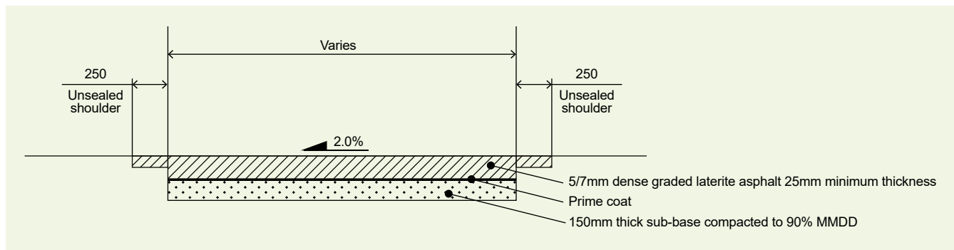
Figure 5.3 Typical pavement cross-section for asphalt paths.
