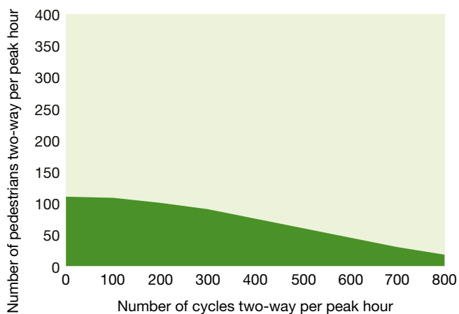
Figure 2.3 Separation criteria for path with 50:50 directional split – typical of paths which are popular with recreational users (image adapted from Queensland Department of Transport and Main Roads 2015).
